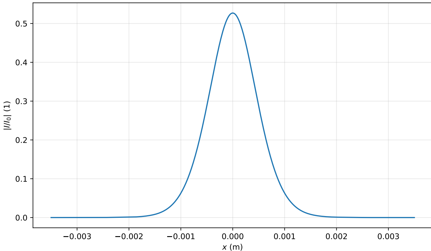
Intensity profile I(x, y = 0, z = 3.184m)/I_0 , P_{in}=0.5P_{cr} , artificial time
